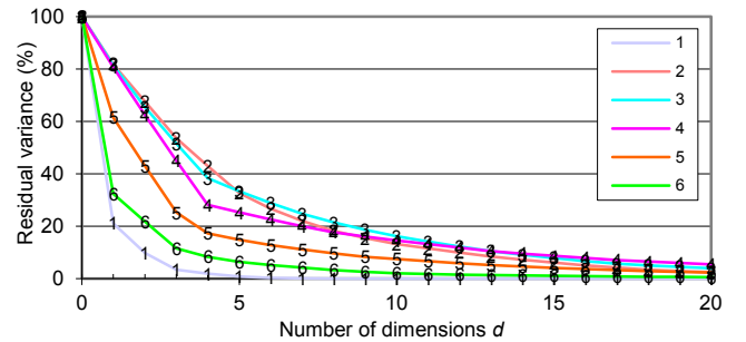
Figure 15: Appearance-space variance unaccounted by the largest d=1 \dots 20 principal components, for synthesis levels 1-6.
