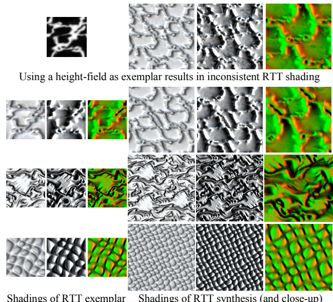
Figure 7: Diffuse radiance transfer as appearance vector, to obtain consistent self-shadowing during RTT shading.
