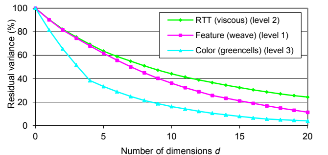
Figure 16: Comparison of appearance-space residual variance for a color texture, a texture with feature distance, and an RTT.
